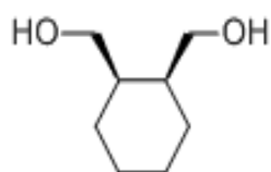
cis-1,2-Cyclohexandimethanol
