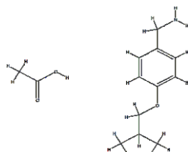
4-(2-Methylpropoxy)benzenemethanamine acetate (1:1)
