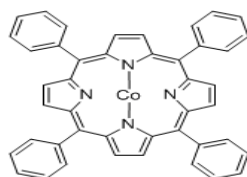
Cobalt(II) Tetraphenylporphyrin
