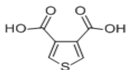
THIOPHENE-3,4-DICARBOXYLIC ACID
