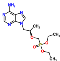
(R)-9-[2-(Diethylphosphonomethoxy) propyl]adenine
