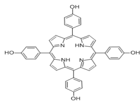
5,10,15,20-TETRAKIS(4-HYDROXYPH ENYL)-21H,23H-PORPHINE
