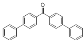
4,4'-DIPHENYLBENZOPHENONE
