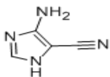
5-Amino-1H-imidazol-4-carbonitrile
