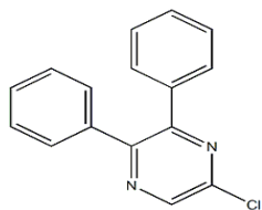
5-chloro-2,3-diphenylpyrazine
