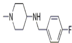
N-[(4-Fluorophenyl)methyl]-1-methyl-4-piperidinamine
