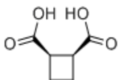
CIS-CYCLOBUTANE-1,2-DICARBOXYLIC ACID
