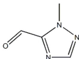
2-Methyl-2H-[1,2,4]triazole-3-carba ldehyde
