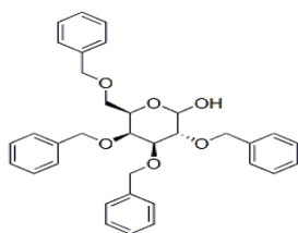
2,3,4,6-TETRA-O-BENZYL-D-GALACTOPYRANOSE
