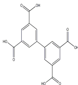
[1,1'-biphenyl]3,3',5,5'-tetracarboxylic acid
