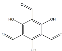
2,4,6-Trihydroxy-benzene-1,3,5-tric arbaldehyde
