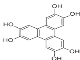
triphenylene-2,3,6,7,10,11-hexaol
