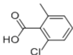
2-CHLORO-6-METHYLBENZOIC ACID
