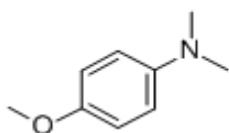
4-Methoxy-N,N-dimethylaniline
